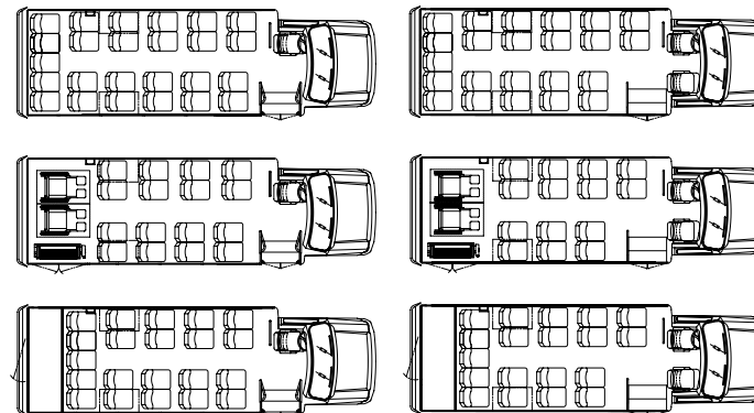
Single Door Floor Plans
